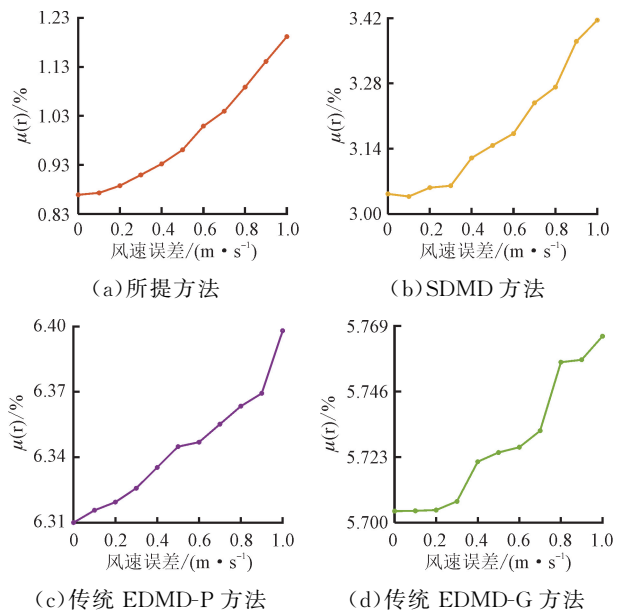
图 4 风速误差下不同方法所建模型的风轮转速预测误差 Fig. 4 Prediction errors of models established by different methods under wind speed errors
